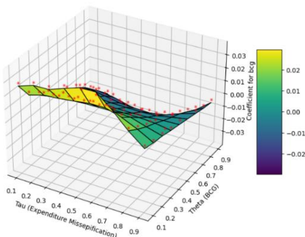
3D Plot of Coefficients for bcg
